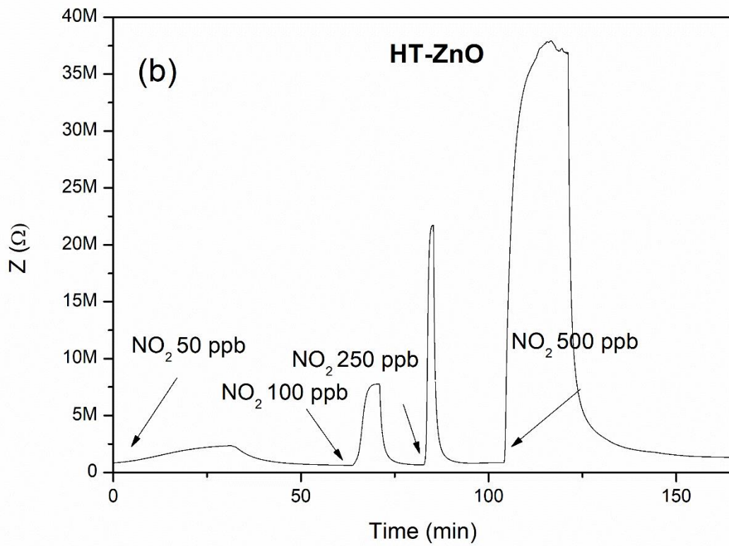
Fig. 7 Impedance's variations of (a) AC-ZnO sensor and (b) HT-ZnO sensor upon different \text{NO}_2 concentrations exposure at 150^\circ\text{C} .
