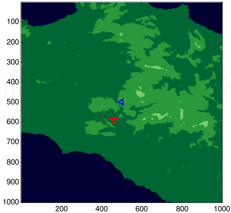
Fig. 10. Digital Elevation Map of the western part of Sicily showing the Bisacchino radar site (red triangle) and the Giuliana rain gauge location (blue triangle). Axes map units are 90-m pixels.
