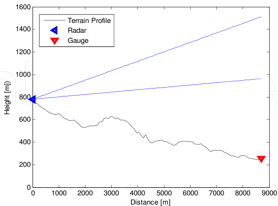
Fig. 11. As in Fig. 6, but for the Bisacchino radar and the Giuliana rain gauge.
