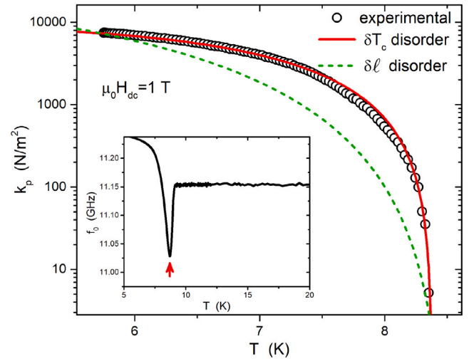
Fig. 7. Pinning constant k_p as a function of temperature, for an applied dc field of 1 T. The red line is the behavior expected for \delta T_c pinning, according to Eq. (5), while the green dashed line shows what would be the temperature dependence in the case of \delta \ell pinning. In the inset, the observed f_0(T) anomaly is reported. (For interpretation of the references to color in this figure legend, the reader is referred to the web version of this article.)
