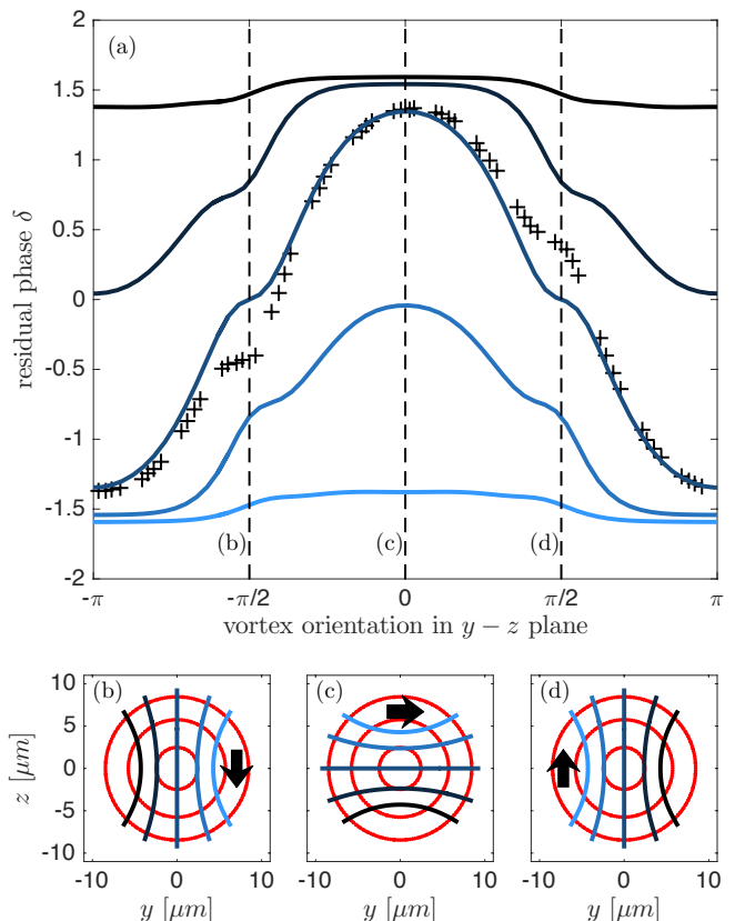
Figure 7. (a) Numerically determined residual phase \delta after a 10 ms partial expansion as a function of in situ vortex orientation. Solid curves are for untilted (strictly in the x = 0 plane) vortices while the '+' symbols are for the tilted precessing vortex already shown in Fig. 6 (a). The middle curve is for a vortex that runs through the origin while the others are for off-center vortices. The three dashed lines mark when the untilted vortices are oriented along the vertical ( -z ), horizontal ( +y ) and vertical ( +z ) direction, and these correspond to the examples in the lower panels that illustrate the positions of the off-center vortices. (b)-(d) Cuts through the x = 0 plane illustrating the positions of the vortex cores in the main plot. Density isocontours are at 10%, 50% and 90% of the peak density. The arrows indicate the sense of vorticity. Note that the curves in the upper and lower subplots have a matching color code to guide the eye.
