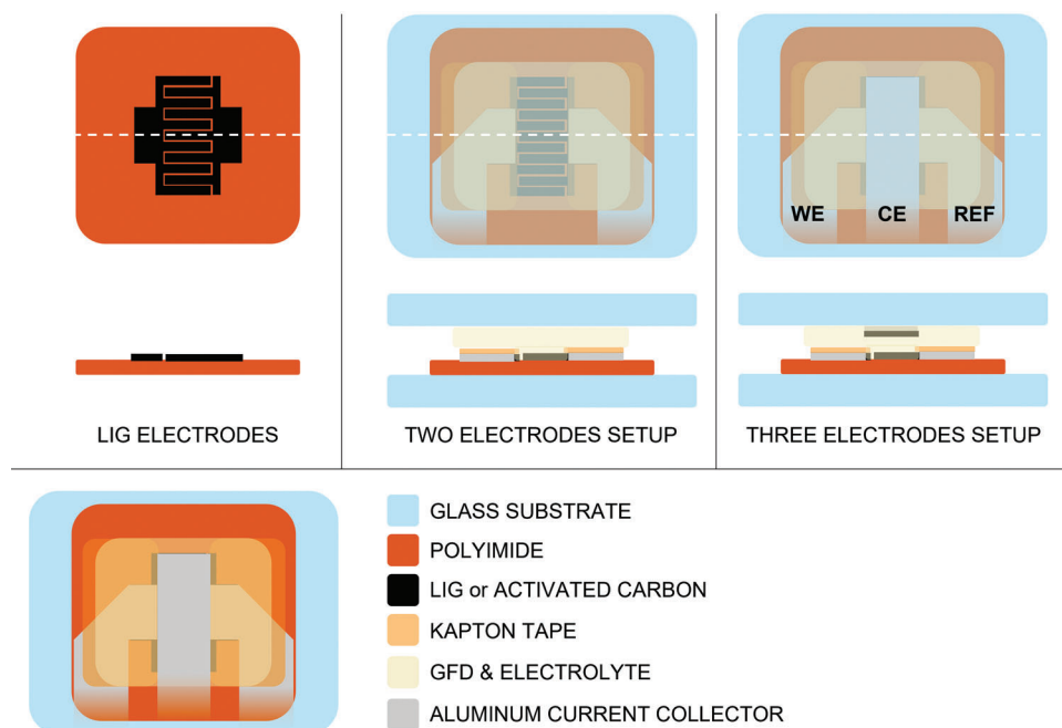
Figure 2. Printed LIG electrodes. Electrochemical cell architectures for the device and the three electrodes setups.
