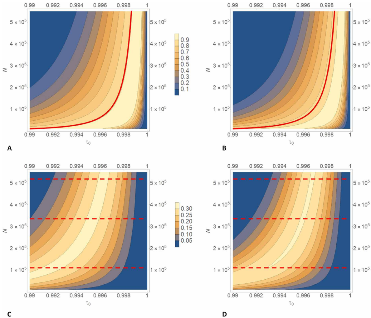
Fig. 2. Information gain G of quantum reading as a function of the lower transmissivity \tau_0 and total mean number of photons N (higher transmissivity is set to \tau_1 = 1 ). The information gain is computed assuming a TMSV-state transmitter with large number of copies ( M \approx 10^{13} ) and a receiver based on photon counting. In (A), the classical benchmark is the photon-counting performance with classical states of Eq. 6. In panel (B), the benchmark is the optimal classical limit in Eq. 1. In both panels, the red curve represents the MED strategy described in the text, marking the limit after which the channels are classically indistinguishable. In (C) and (D), we consider the case of imperfect quantum efficiency \eta = 0.76 for both the signal and idler systems (so that \tau_u \rightarrow \eta\tau_u for u = 0, 1 ). We show the gain over the photon-counting classical bound in (C), and the gain over the optimal classical limit in (D). In (C) and (D), the dashed lines indicate the regions where experimental data were collected. These data points are those reported in Fig. 4.
