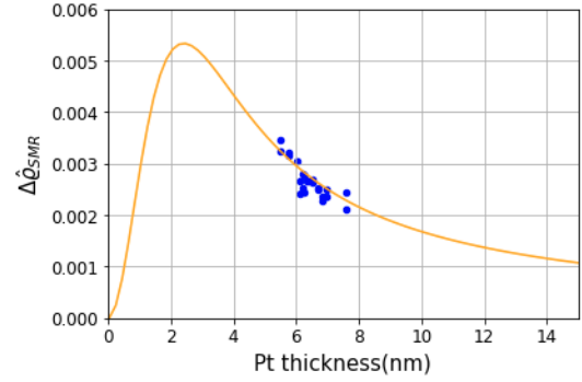
Fig. 5. \Delta \hat{Q}_{SMR} as a function of Pt thickness. Blue points: measured data. Yellow curve: fit following (3) using G_c = 1 \cdot 10^{16} \Omega^{-1}m^{-2} , \theta_{SH} = 0.14 , and l_{Pt} = 1.1 nm.
