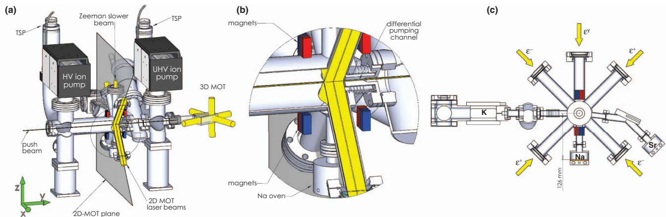
FIG. 1. (a) 3D view of the vacuum system. HV region on the left side contains the atomic source and the optical access for the pre-cooling stage. The differential pumping channel connects this to the UHV region where the experiment is performed in a clean environment. Light beams (yellow) and magnets (red-blue) are shown. (b) Magnification of the compact slowing/cooling region. (c) 2D view of the pre-cooling plane showing atomic sources and beams configuration.
