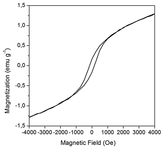
Figure 7. Magnetisation curves at 300 K of RED-NH 2 -Fe-SBA-15 sample.
