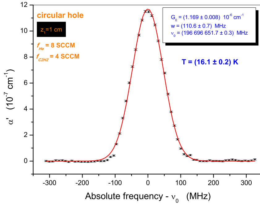
Fig. 6 CRDS signal measured on the acetylene beam for f_{\text{C}_2\text{H}_2} = 4 sccm and f_{\text{He}} = 8 sccm at a distance of z_1 = 1 cm from the BGC cell exit. Here, the escape hole is circular with a diameter of 2 mm. Thanks to the enhanced signal-to-noise ratio ( SNR \simeq 250 ), the center frequency of the (\nu_1 + \nu_3) R(1) ro-vibrational line is now measured with a fractional accuracy of 1.5 \cdot 10^{-9} .
