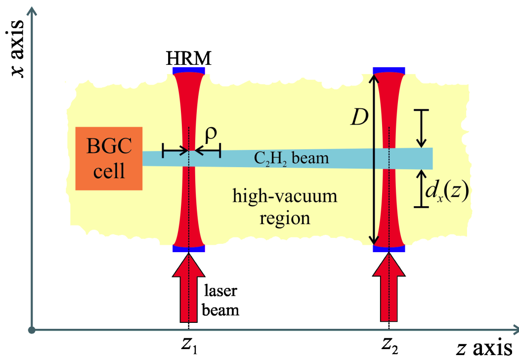
Fig. 4 Schematic topview (not to scale) of the CRDS setup evidencing the relevant geometrical parameters involved in the estimation of the molecular beam density and divergence.
