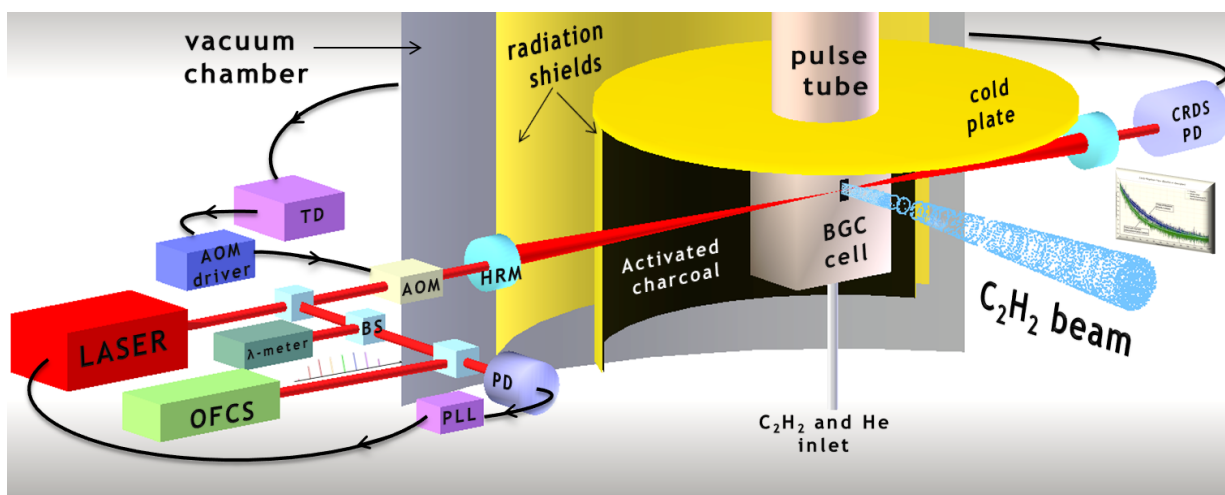
Fig. 1 Layout of the experimental setup consisting of two main blocks: the buffer-gas-cooling source and the comb-referenced laser spectrometer. The following legend holds: HRM=high-reflexivity mirror, TD=threshold detector, PD=photo-detector, PLL=phase locked loop, BS=beam splitter.
