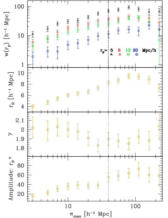
Fig. 5. Upper panel: projected correlation function w(r_p) computed at different r_p scales (see label) as a function of the integration radius \pi_{\text{max}} . From top middle to bottom panels the correlation length r_0 , slope \gamma , and amplitude r_0^\gamma are shown as a function of \pi_{\text{max}} , respectively.
