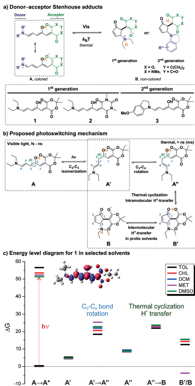
Figure 1. Donor–acceptor Stenhouse adducts: a) photoswitches used herein; b) proposed photoswitching mechanism [15,16] and c) corresponding energy level diagram in kcal mol −1 for 1 in selected solvents obtained at the M06-2X/6-31 + G(d)/SMD level of theory. Analogous diagrams for 2 and 3 are presented in the SI (Figure S8.5). In the electronic density difference (EDD) plot (inset), the blue (red) regions correspond to a decrease (increase) in electron density upon electronic excitation. The energy levels of the product correspond to B and B' structures in protic and aprotic solvents, respectively.
