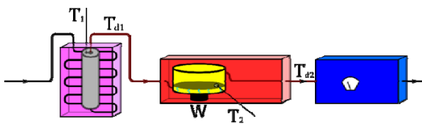
Fig. 13. Schematic diagram of the sorption isotherm measurement systems developed at DTI. T_1 =saturator temperature, T_{d1} =dew-point temperature at the saturator outlet, T_2 =air temperature in sample chamber, T_{d2} =dew-point temperature at the hygrometer inlet, W = weight of the sample continuously monitored by a scale.
