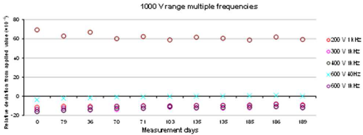
Fig. 8. Deviations in the 1000 V range at multiple frequencies for AC Voltage.
