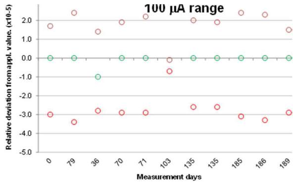
Fig. 10. Deviations in the 100 \mu A range for DC Current.
