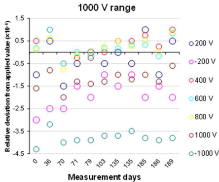
Fig. 5. Deviations in the 1000 V range for DC Voltage.
