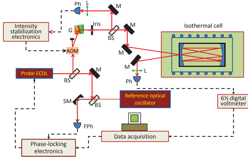
Figure 1. (Color online) Sketch of the dual-laser spectrometer. BS: beam splitter; M: mirror; SM: spherical mirror; G: grating; L: anti-reflection coated lens; AOM: acousto-optic modulator; Ph: InGaAs photodiode; FPh: fast photodiode.
