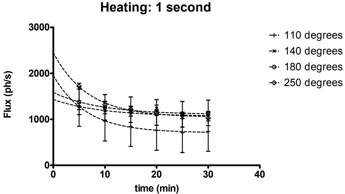
Fig 4 The plot show the decay of the HIL signal and the corresponding fitting (dotted line) for the different temperatures and a heating time equal to 1 second. The heating was obtained with a welding device.
