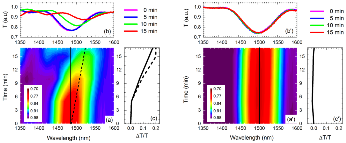
Figure 5: Optical response to toluene vapor exposure of DBR sensors. Nanocomposite DBR on the left and control DBR on the right. a, a') Contour plot of the transmittance spectra collected every 5 minutes; b, b') Corresponding transmittance spectra; c, c') Time dependent differential transmittance at initial photonic band gap wavelength (solid line in panel a and a') and minimum of transmission (dashed line in panel a).
