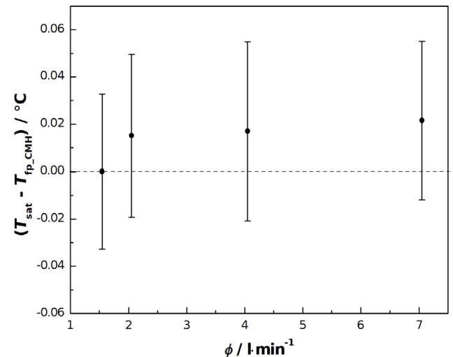
Figure 10. Differences between the saturated gas temperature, T_{\text{sat}} , and the frost-point temperature measured by the CMH, T_{\text{fp\_CMH}} , as a function of the flow rate, \phi . Reported data refer to a gas pressure of about 1100 hPa and a saturated gas temperature of about -75^\circ\text{C} .
