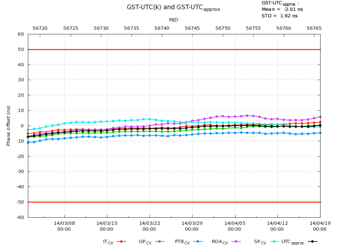
Fig. 2. GST-UTCapprox evolution over one and a half months.
