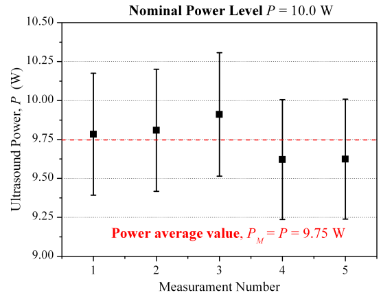
Fig 2. Ultrasound Power emitted from Device 1 Probe 1 MHz
