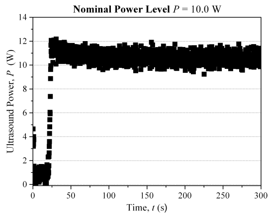
Fig 11. Ultrasound Power vs. time Device Probe 1 MHz
