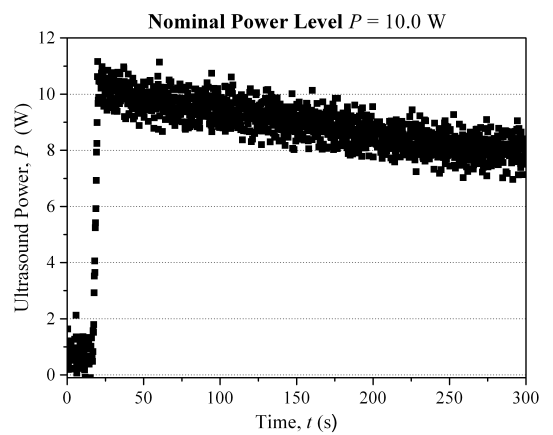
Fig 9. Ultrasound Power vs. time Device 3 Probe 1 MHz
