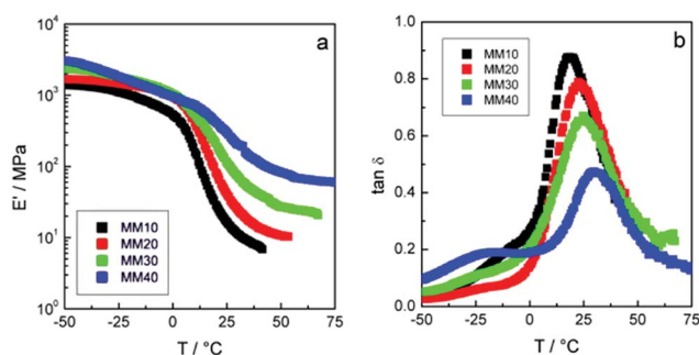
Fig. 2 Trends of E' (a) and \tan \delta (b) for the films prepared by mixtures MM10 – MM40 analyzed along the direction parallel to the liquid crystalline alignment.
