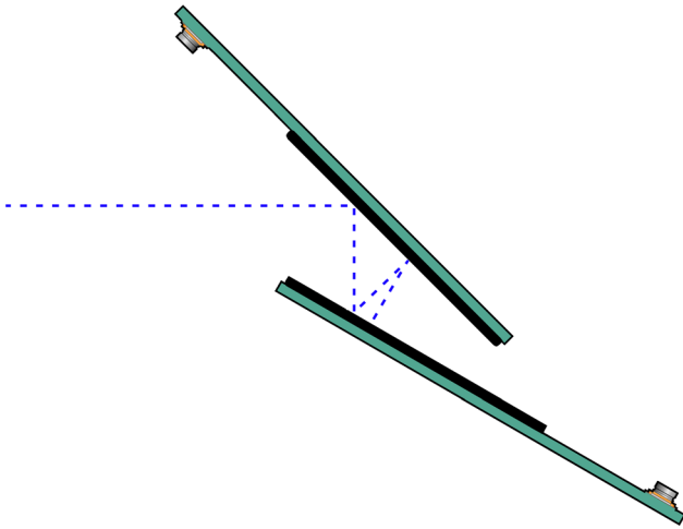
Figure 3. Schematic drawing of the light-trapping assembly. The angle between the photodiodes is 15^\circ for the seven-reflection trap structure and 11.25^\circ for the nine-reflection structure.
