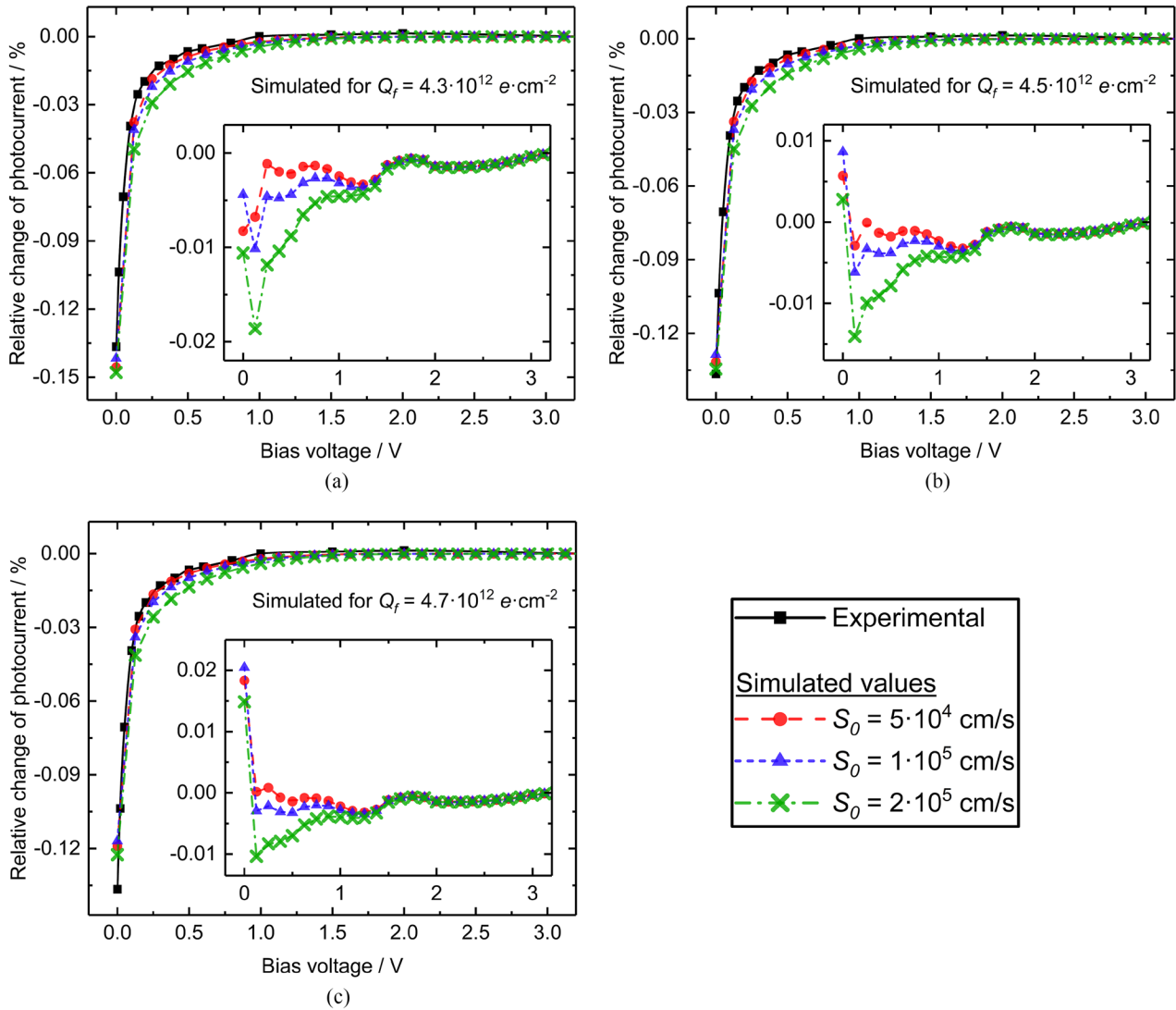
Figure 9. Measured and simulated relative change of photocurrent for Set B photodiodes. The simulations are shown for Q_f values of 4.3 \cdot 10^{12} \text{ e cm}^{-2} (a), 4.5 \cdot 10^{12} \text{ e cm}^{-2} (b) and 4.7 \cdot 10^{12} \text{ e cm}^{-2} (c). The inserts show the deviations of simulated values from cubic spline interpolation of the measured values.
