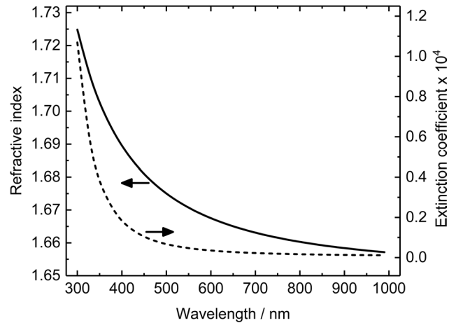
Figure 4. Refractive index and extinction coefficient of the ALD grown \text{Al}_2\text{O}_3 layer of the n -type PQED photodiode.
