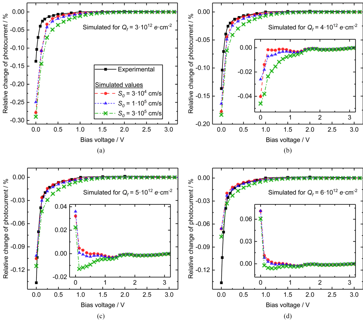
Figure 8. Measured and simulated relative change of photocurrent as a function of bias voltage for Set B photodiodes. The simulations are shown for Q_f values 3 \cdot 10^{12} \text{ e cm}^{-2} (a), 4 \cdot 10^{12} \text{ e cm}^{-2} (b), 5 \cdot 10^{12} \text{ e cm}^{-2} (c) and 6 \cdot 10^{12} \text{ e cm}^{-2} (d). The inserts show the deviations of simulated values from cubic spline interpolation of the measured values.
