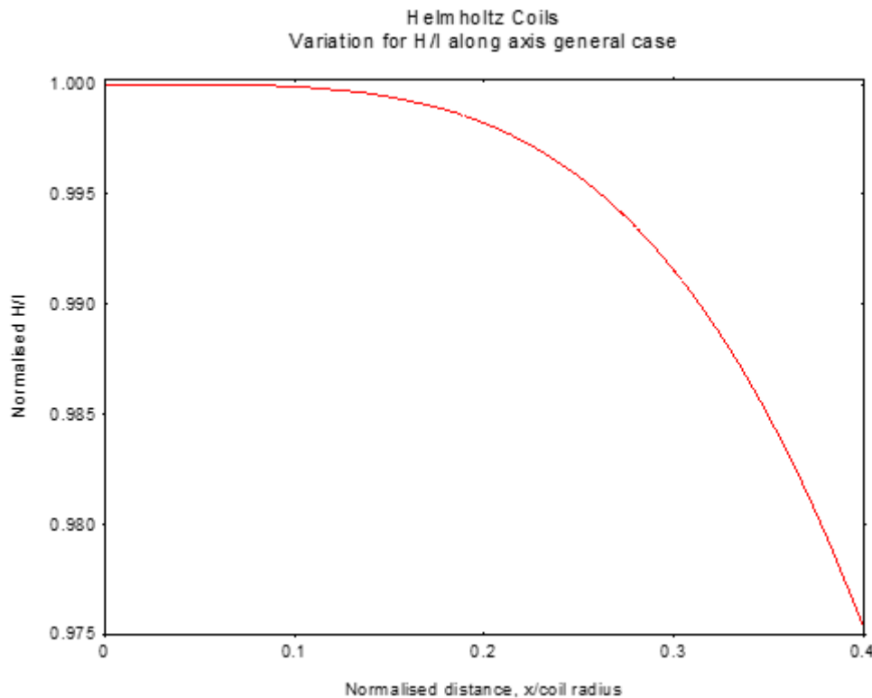
Figure 9. Variation of H/I along the X-axis (axis through the centre) of the coils.
