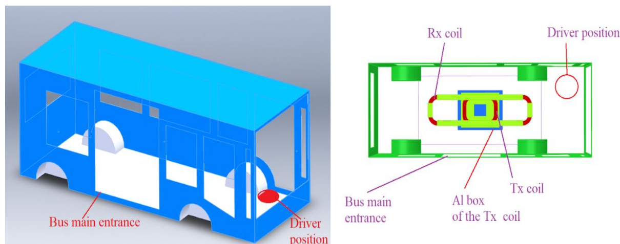
Figure 16. Bus body: a) 3D representation, b) plan view. The Tx coil size is 0.8 m x 0.6 m and the on-board Rx coil is 2.5 m x 0.6 m. The total length of the bus is 5.1 m, while the total width is 2.3 m.
