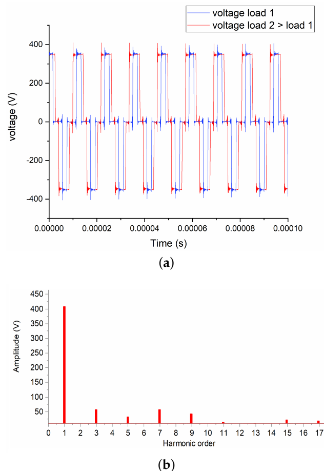
Figure 9. (a) Voltage at LVCS transmitter coil (two load conditions). (b) FFT spectrum of the voltage in the resonant circuit (load 2 in Figure 8a).
