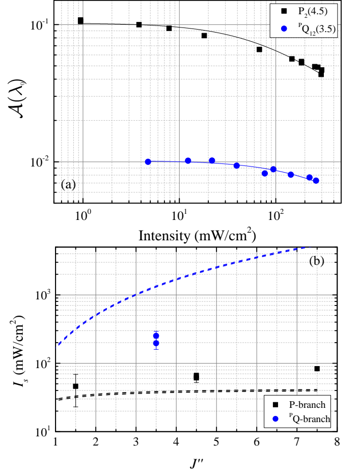
FIG. 10. Experimental study of the transient saturation intensity on a BaH molecular plume for different rovibrational transitions. (a) The fractional absorption versus probe laser intensity for the P_2(J = 4.5) and P_{12}(3.5) lines. (b) Summary of all the I_s measurements on the P (black squares) and PQ (blue circles) branches of the B - X (0,0) band. Comparison lines with the expected values according to Eq. (8) are drawn.
