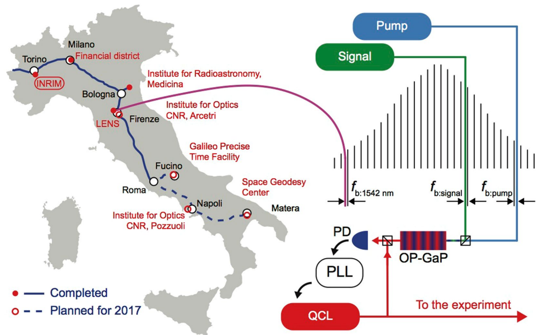
Figure 1. The left part of the figure shows the Italian fibre link network, blue line, with network nodes in red. At LENS/University of Florence (LENS in the following for brevity), the ultra stable laser at 1542 nm locks the repetition rate of a frequency comb. We measure the beat notes of two near-IR lasers against the frequency comb and keep their frequency difference constant with an indirect locking scheme to cancel out the comb noise contribution 29 . The two lasers are combined in an OP-GaP crystal to generate mid-IR light, to which we lock a quantum cascade laser. (The map is obtained on the basis of ©OpenStreetMap contributors ( www.openstreetmap.org ) licensed under the Creative Commons Attribution-ShareAlike 2.0 license (CC BY-SA) https://creativecommons.org/licenses/by-sa/2.0/ . The basis was then modified to fit our figure and we took no care to maintain proportions or accuracy).
