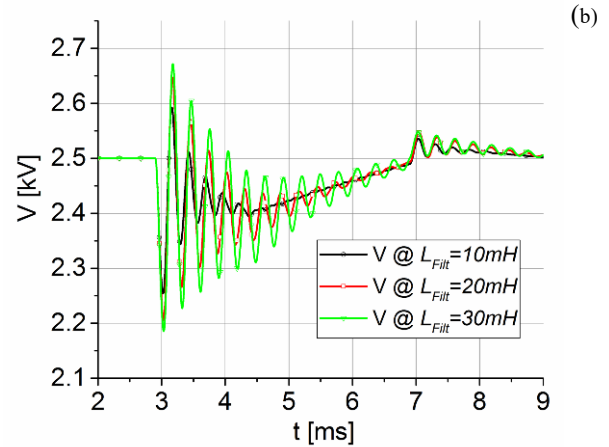
Fig. 18. Effect of the OHL resistance R_{OHL-DC} on the estimated voltage at the output of the measurement chain a). Effect of the inductance filter L_{filt} value on the estimated voltage at the output of the measurement chain b)
