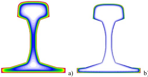
Fig. 20. Map of the magnetic induction strength for a 50 Hz injected current signal a) and for a 2 kHz current signal b)
