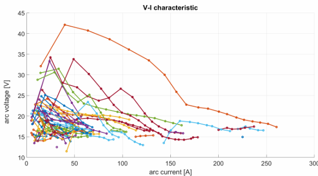
Fig. 8. Collection of volt-ampere characteristic for random arc events
