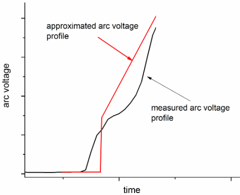
Fig. 15. Time behaviour, in the initial part of the event measured and approximated
