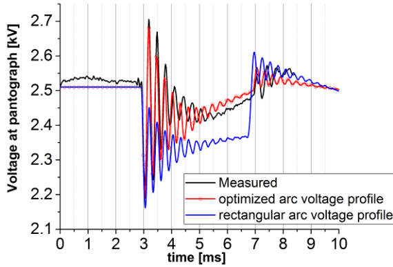
Fig. 19. Comparison between voltages measured at the pantograph and simulated one
