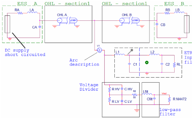
Fig. 14. Circuit model for the analysis of arc conducted effects
