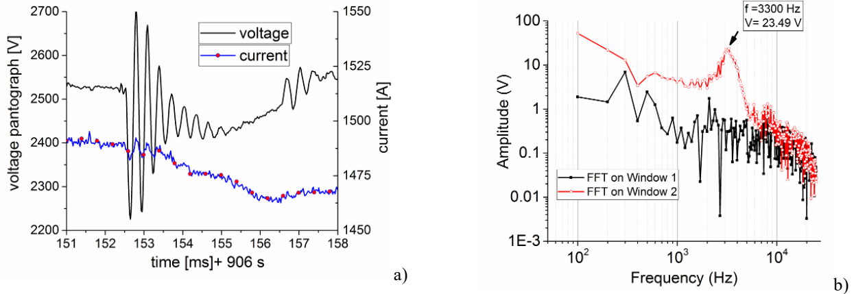
Fig. 13. Time domain zoom of the pantograph voltage and current during the transient oscillation a). Spectrum of the pantograph voltage before (window 1) and during (window 2) the transient oscillation b)
