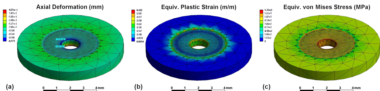
FIG. 6. Mechanical FEA of the gasket: (a) axial deformation; (b) equivalent plastic strain; (c) equivalent von Mises stress. FEA calculations predict an appreciable plastic deformation of the gasket at the anvil contact region, with an indentation of about 0.17 mm, very close to the experimentally measured value of 0.20 mm. At this location, the equivalent von Mises stress exceeds the yield stress of the gasket, here corresponding to 900 MPa.
