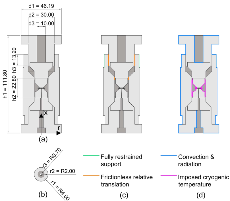
FIG. 4. (a) Longitudinal cross section of the pressure cell showing the main dimensions in a load-free condition: h_1 is the total length; h_2 is the distance between top and bottom surfaces of the anvils; h_3 is the free sliding length between the upper locknut and the body, which are characterized by frictionless contact; d_1 is the maximum external diameter of locknuts; d_2 and d_3 indicate locknut and pusher diameters. (b) Top view of the gasket with main dimensions (maximum size): for all the gasket sizes, the outer radius r_1 is equal to 4 mm, whilst, for the largest gasket, the inner radius r_3 is equal to 0.7 mm and the radius of the indented region r_2 is equal to 2 mm. (c) Mechanical boundary conditions: the fully restrained support simulates the fixation of the pressure cell, constrained by a stiff aluminum cylinder (omitted in this picture); the frictionless contact condition allows for the relative translation of the upper locknut and body owing to piston pre-load. (d) Thermal boundary conditions: convection and radiation simulate heat exchange with the surroundings, whilst the imposed cryogenic temperature takes into account the effect of a heater-thermometer coupled system fixed on the outer surface of the body, close to the inspection hole, to enhance the control of the sample temperature. All the dimensions are in mm.
