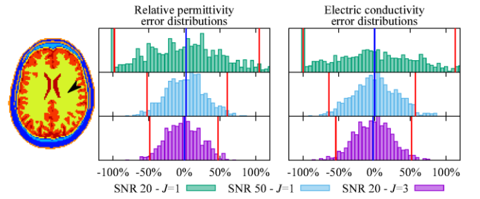
Fig. 4. Relative frequency histograms of electric properties relative errors after 300 iterative steps in the inner pixel identified by the arrow in the map on the left. A 16 legs birdcage coil is considered with different coil settings and different amount of noise. The vertical blue lines denote the relative errors in absence of noise; the vertical red lines indicate the shortest 95 % coverage intervals.
