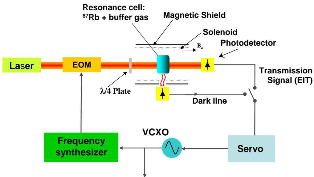
Fig. 6. – Schematic setup of the CPT clock based on the dark line or on the EIT signals. EOM: Electro-optic modulator. VCXO: Voltage Controlled Crystal Oscillator. Laser stabilization and thermal controls not shown in the figure.
