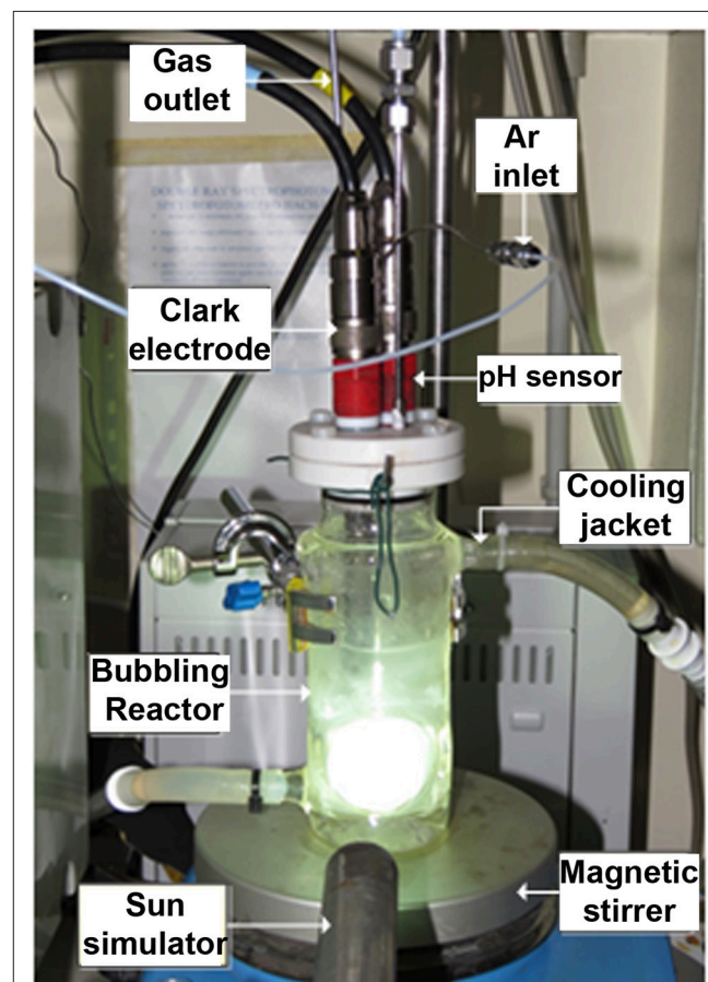
FIGURE 1 | Photocatalytic bubbling reactor used for the water oxidation experiments.
