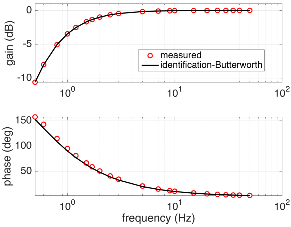
Fig. 4. Result of the fitting with cut-off frequency equal to f_{\text{cut}} = 1 Hz. Measured frequency response vs. Butterworth frequency response.
