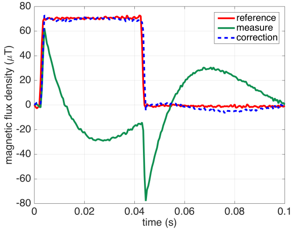
Fig. 10. Test of the correction procedure on the measured waveform with f_{cut} = 10 Hz. The red curve is the reference waveform, the green curve is the waveform measured by the meter and the blue (dashed) curve waveform obtained by means of the correction procedure.
