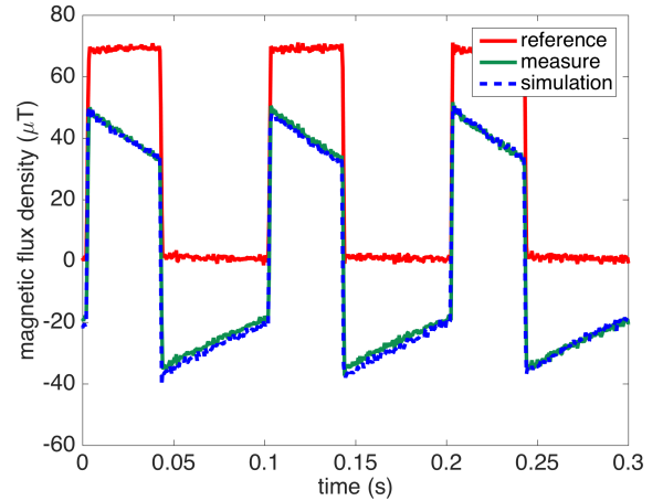
Fig. 6. Simulation of the measurement artefact related to f_{\text{cut}} = 1 Hz. The red curve is the reference waveform, the green curve is the waveform measured by the meter and the blue (dashed) curve is the simulation.
