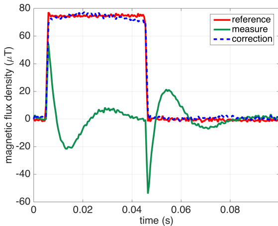
Fig. 11. Test of the correction procedure on the measured waveform with f_{cut} = 30 Hz. The red curve is the reference waveform, the green curve is the waveform measured by the meter and the blue (dashed) curve waveform obtained by means of the correction procedure.
