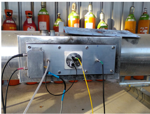
Fig. 4. Photo of the parts installed on the stack. The preamplifier is inside the metallic box on the left.
