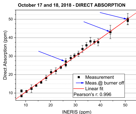
Fig. 10. Correlation of direct absorption measurements with INERIS FTIR analyser.
