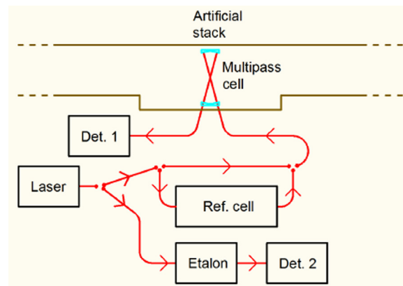
Fig. 5. Block diagram of the optics.
