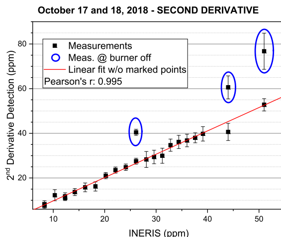
Fig. 11. Correlation of second derivative measurements with INERIS FTIR analyser.
