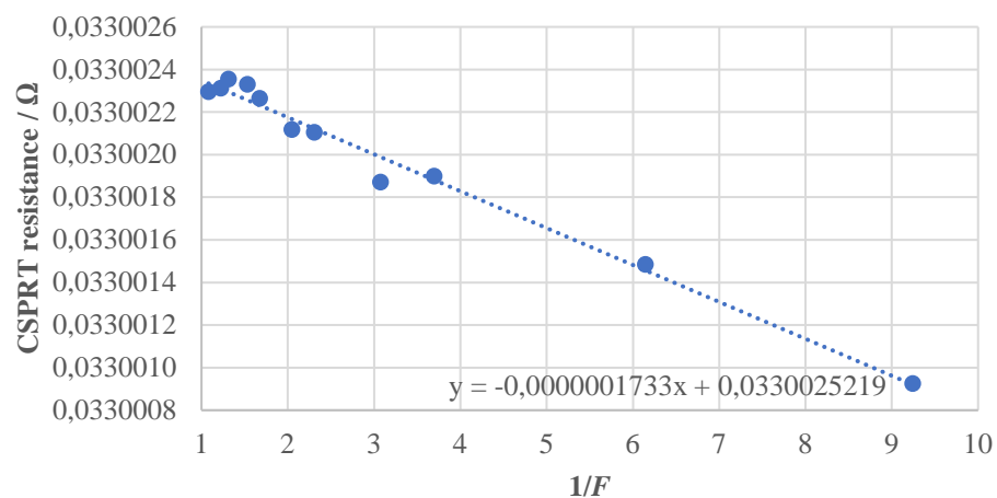
Figure A.4 The resistance values of the CSPRT measured after each heat pulse, reduced to zero current, are finally plotted against the calculated values of 1/F and extrapolated to F = 1 (N.B.: the temperature difference between the outer points is about 0.224 mK). After correction for the isotopic effect, the final value of resistance R at the triple point is given.
