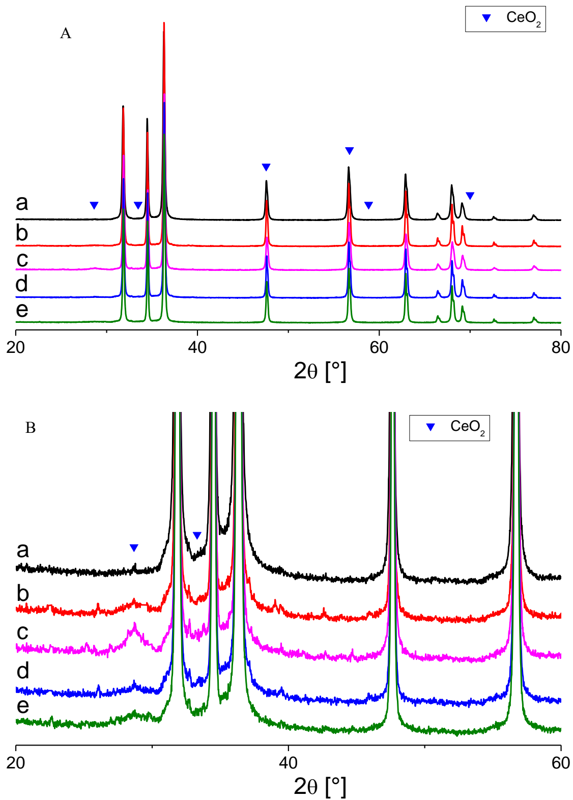
Fig. 1. XRPD patterns of (a) ZnO, (b) Ce 0.05 Cl, (c) Ce 0.1 Cl, (d) Ce 0.05 S and (e) Ce 0.1 S. Panel B is a magnification of panel A.
