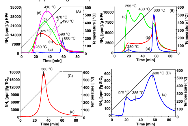
Figure 1. Temperature programmed desorption curves of ammonia ( NH_3 -TPD) for the as prepared samples: (A) PW_{12} (a); PW_{12}/N-TiO_2 (b); PW_{12}/TiO_2 (c); PW_{12}/TiO_2 ex A (d); (B) PW_{12} (a); PW_{12}/SiO_2 (b); PW_{12}/SiO_2 ex A (c); (C) TiO_2 (a) and (D) SiO_2 (a).
