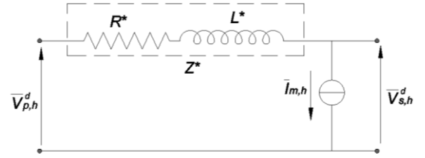
Fig. 1. Equivalent circuit of VT at h -order harmonic frequency.
