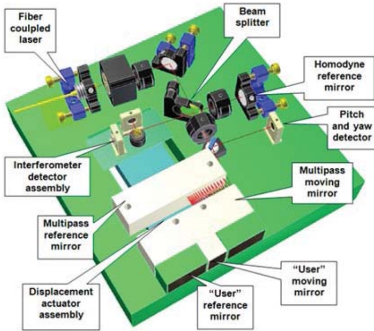
Fig. 6. Rendering of the PRA main components: the actuator relies on a multiple reflection interferometer as a traceable measurement of the mirror displacement.
