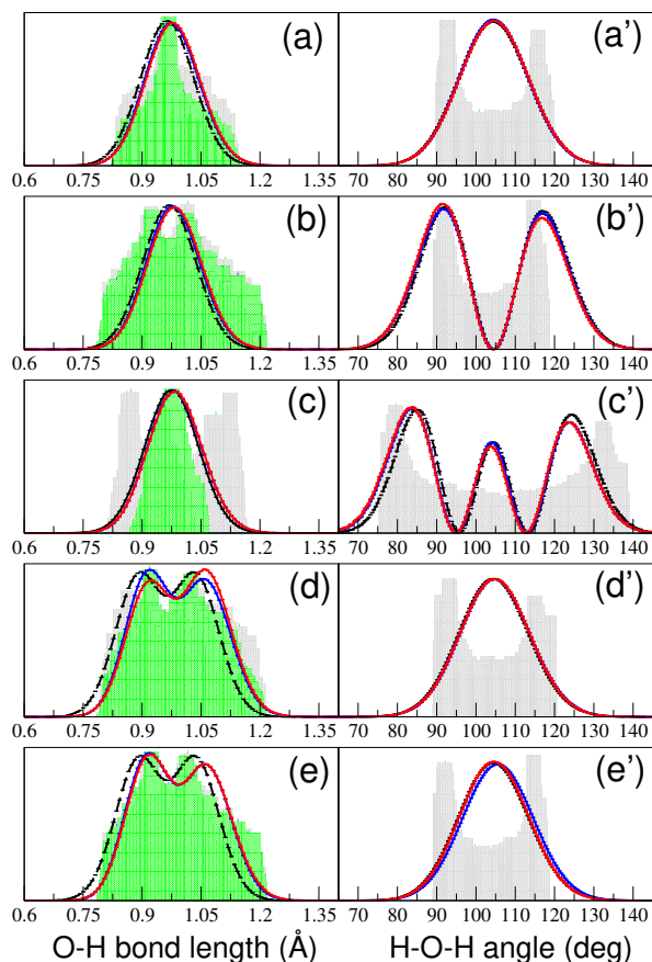
Figure 3. Water bonds and H-O-H angle probability density distributions obtained from quantum harmonic (black dashed line), DVR 39 (blue line), and semiclassical (red line) wavefunctions. Left panels (a), (b), (c), (d), and (e) are respectively for the radial O-H distribution of the ground (000), (010), (020), (100) and (001) vibrational eigenfunctions. Right panels (a'), (b'), (c'), (d'), and (e') are for the angular H-O-H distributions of the same ordered vibrational states. The filled-area plots on the background represent the classical distributions obtained from the classical trajectory used to generate each wavefunction with our semiclassical approach. In the left panels, gray and green histograms stand for the two bond-length distributions along each water O-H bond and, in the right panels, gray histograms are for the H-O-H angle.
