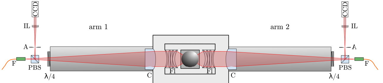
Figure 2. Schematic of PTB set-up; F: fibre, PBS: polarising beam splitter, A: aperture, CCD: camera (512 × 512 pixels), IL: imaging lens, C: Collimator, FL: Fizeau lens.
