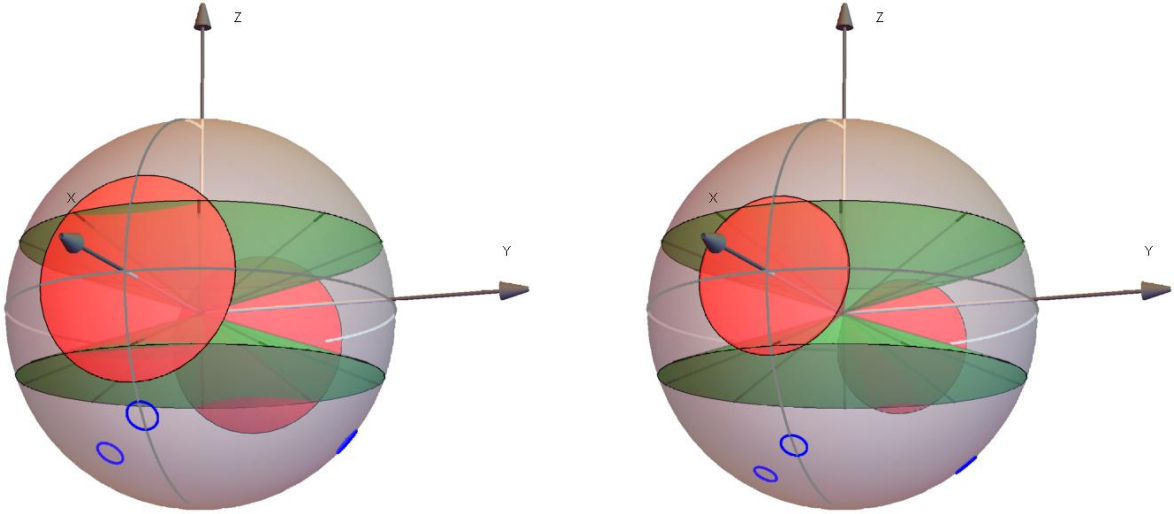
Figure 3. Measurement geometries of the PTB's interferometers 1 (left) and 2 (right). The supporting pins (blue circles) are at 40° (left) and 50° south (right) latitude and spaced by 120° azimuth. The zero meridian (grey) goes through the first pin and beam axis. The azimuths are positive in the counterclockwise direction. The measured diameters are inside the red cones having 60° (left) 45° (right) apertures. The green cones are the diameters at 20° north latitude whose deformation is shown in Figs. 6 and 8.
