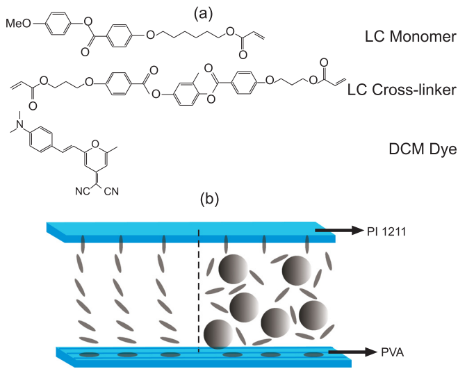
FIG. 1. (a) Chemical structure of the monomer, cross-linker, and dye molecule used to fabricate the composite random laser. (b) Schematic of the random laser: in the left half, the liquid crystals are aligned in the splayed fashion, and in the right half, the TiO 2 nanoparticles are dispersed to provide increased scattering.
