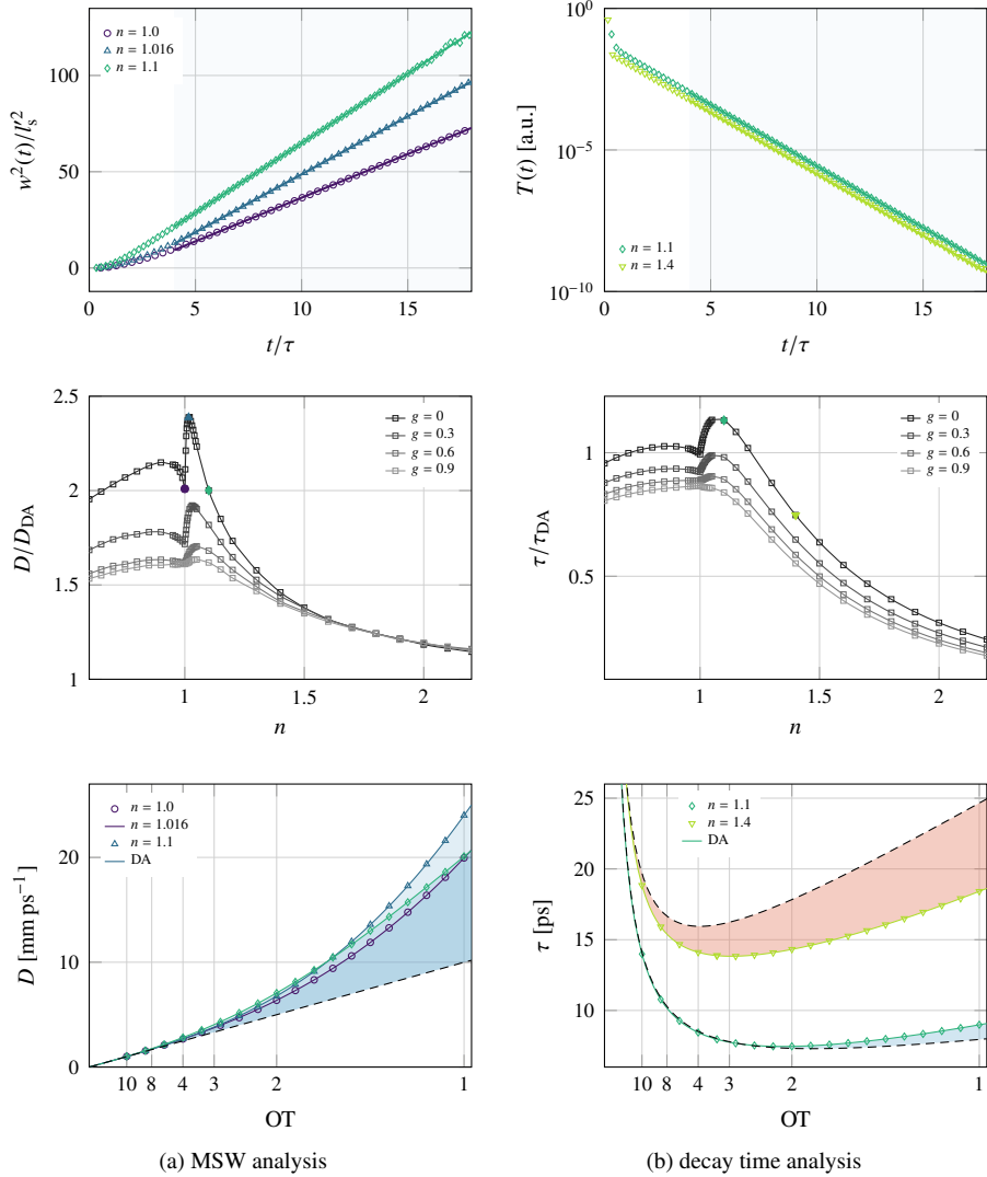
Figure 6.1. From top to bottom: MSW expansion rate and decay time for a slab configuration with l_s = L_0 , g = 0 and different refractive index contrasts, exhibiting (a) a perfectly linear growth and (b) a monoexponential decay after a short transient. Dependence on n and g of the diffusion coefficient D and decay constant \tau as inferred from a linear fit of w^2(t \geq 4\tau) and \log T(t \geq 4\tau) for different samples with OT = 1 . Solid points represent the values retrieved from the fits shown in the upper panel. Absolute positive (blue) and negative (red) deviations with respect to the DA prediction are shown in the lower panels for different optical thicknesses. Solid lines serve as guides to the eye.
