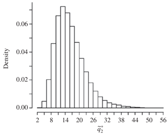
Fig. 5: A histogram of the score \tilde{q}_2^* (%) of effectiveness of the quality system at second step of the ICP-MS analysis (the instrument calibration). This histogram corresponds to judgments of a reasonably doubting expert, simulated by Monte Carlo method. Reproduced from Ref. [18] with permission from Elsevier.
