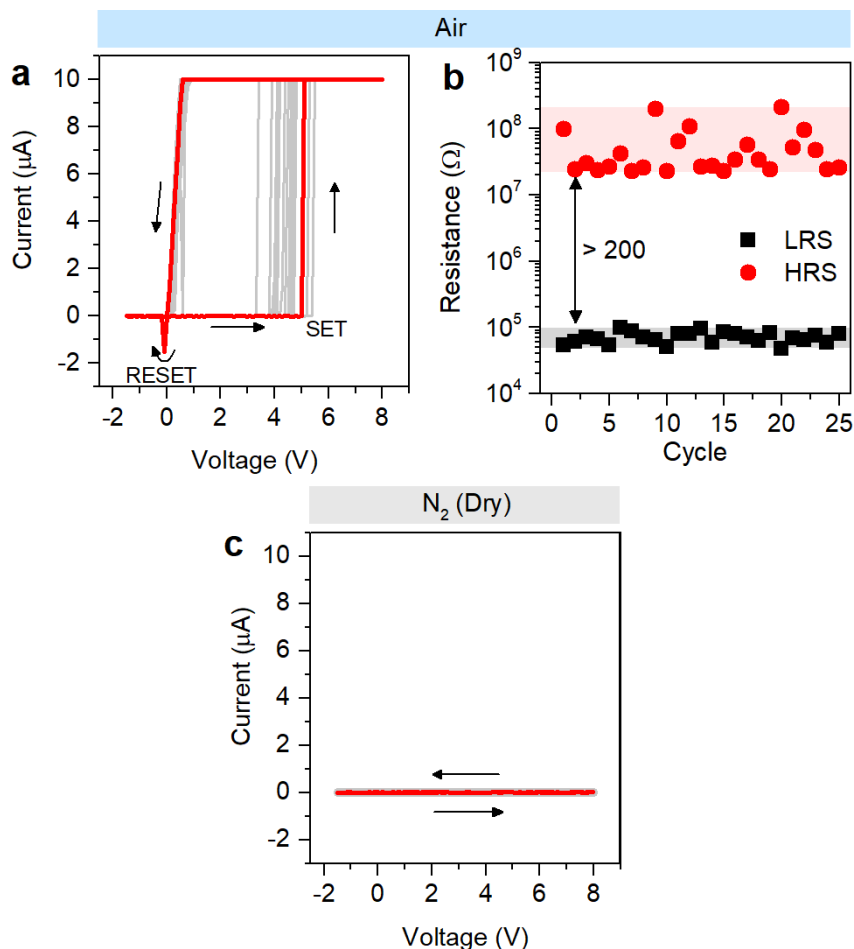
Figure 2. Influence of moisture on resistive switching behaviour. (a) I-V characteristics showing bipolar resistive switching behaviour of a single ZnO NW in air (RH \approx 30 %) and (b) corresponding HRS and LRS values over cycling extrapolated at a reading voltage of 0.4 V. (c) I-V characteristics of the same device in dry air (N 2 environment) showing suppression of the resistive switching behaviour. In both cases, the device was stimulated by means of 25 DC voltage
