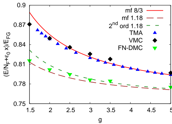
Fig. 2. Energy of a Bose-Fermi mixture with m_B = m_F and x = 0.175 vs. g (with the contribution of the bare binding energy of the molecules subtracted). Full line: mean-field energy (4) with \alpha=8/3 . Long-dashed line: mean-field energy (4) with \alpha=1.18 . Short-dashed line: Eq. (5) with \alpha=1.18 .
