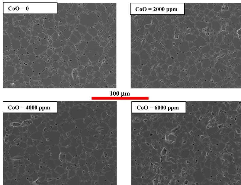
FIG. 1. SEM micrographs of the sintered Mn-Zn ferrites (sintering temperature T = 1325 \text{ }^\circ\text{C} ) with different CoO contents. The average grain size is little affected by addition of CoO (see Table I).
