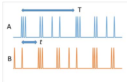
Figure 21: The absolute angle measurement principle. The readings of the two heads have a repetition period T , and are shifted by a time t proportional to the absolute angle between the heads. t is found by autocorrelation function.
