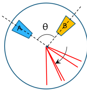
Figure 21: The absolute angle measurement principle. The readings of the two heads have a repetition period T , and are shifted by a time t proportional to the absolute angle between the heads. t is found by autocorrelation function.
