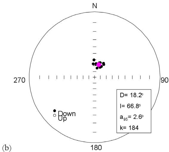
Figure 5 (top and above). (a) Stepwise thermal demagnetization results illustrated as Zijdeveld diagrams for representative samples. Symbols: full dots = declination; open dots = apparent inclination; (b) Equal area projection of the ChRM directions at sample level together with the kiln's mean direction as calculated from Fisher statistics (pink dot).
