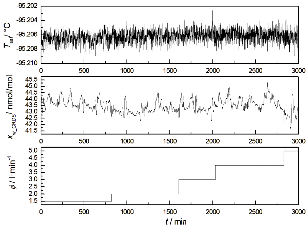
Figure 5. Water vapour amount fraction as measured by the CRDS, x_{w\_CRDS} , as a function of the flow rate, \phi , that ranges between 1.5 and 5 \text{l}\cdot\text{min}^{-1} at operating pressure. The saturation temperature, T_{\text{sat}} is shown in the same time interval. The experiment was carried out at an absolute gas pressure of 800 hPa.
