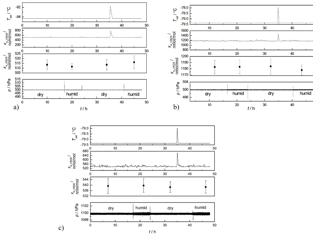
Figure 7. Saturation temperature T_{sat} , water vapour amount fraction x_{w,CRDS} , mean and standard deviations of x_{w,CRDS} and absolute pressure p while alternating the inlet gas between dry ( x_w < 1 \text{ nmol}\cdot\text{mol}^{-1} ) and humid ( x_w > 400 \text{ nmol}\cdot\text{mol}^{-1} ) nitrogen. Panel (a) T_{sat} = -84 \text{ }^{\circ}C and p = 500 \text{ hPa} , (b) T_{sat} = -79 \text{ }^{\circ}C and p = 500 \text{ hPa} , (c) T_{sat} = -79 \text{ }^{\circ}C and p = 1100 \text{ hPa} .
