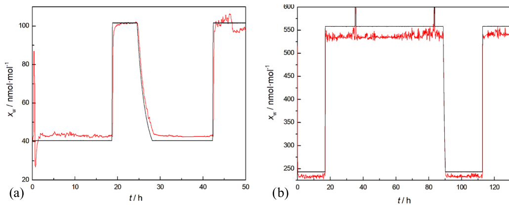
Figure 8. Response of the humidity generator at step changes of the saturation temperature; (a) between -95 \text{ }^{\circ}C and -90 \text{ }^{\circ}C (that is, between 40 and 100 ppb) and (b) between -85 \text{ }^{\circ}C and -80 \text{ }^{\circ}C (that is, between 240 ppb and 550 ppb). Measurements have been carried out at 2 \text{ l}\cdot\text{min}^{-1} at a pressure of 1000 hPa. The red line represents the water vapour amount fraction measured by the CRDS, x_{w,CRDS} ; the black line represents the reference water vapour amount fraction x_{w,0} estimated from the measurement of T_{sat} and p .
