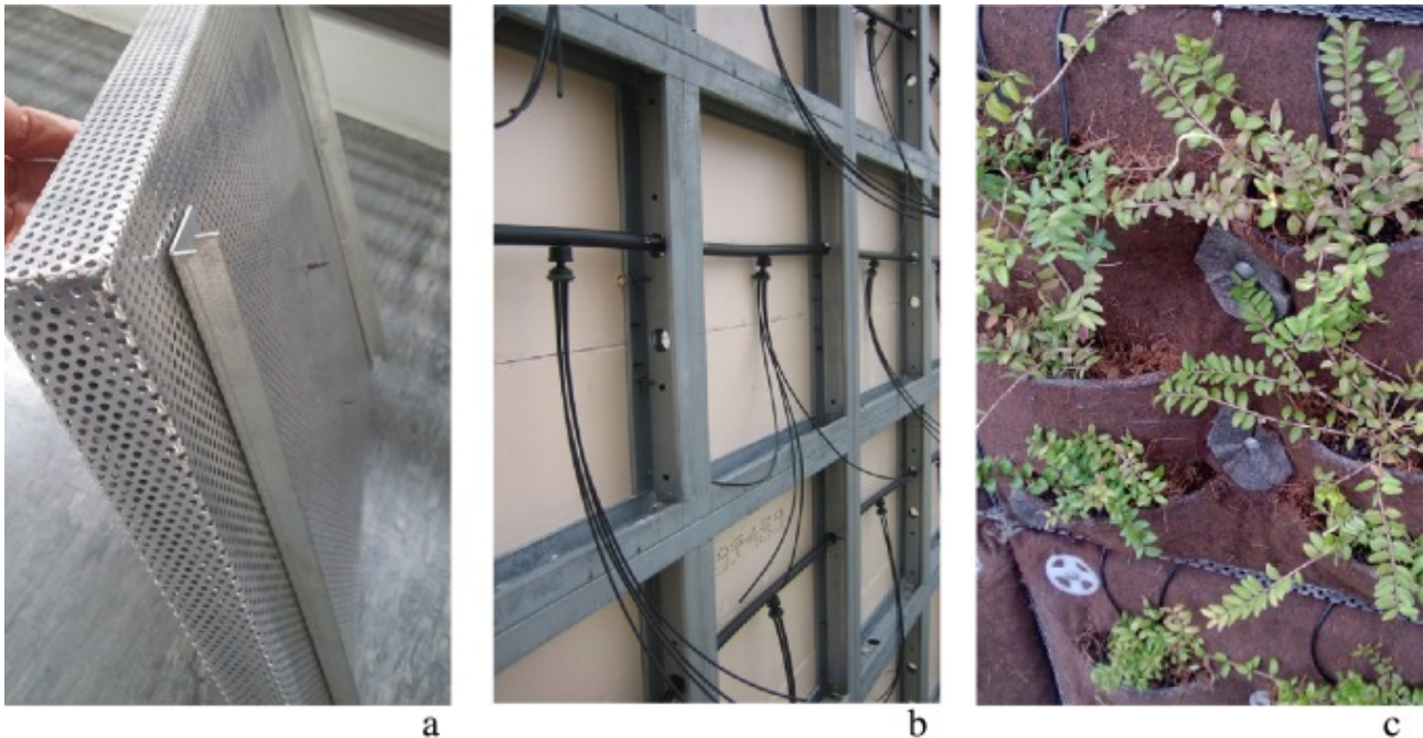
Fig. 3. The reverse assembling connections made up of metal brackets for the anchorage of the modular box to the metal frame (a); the metal frame with the integrated irrigation system (b); the modular box with plants (c).
